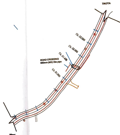
PLAN VIEW ROAD CROSSING-02
