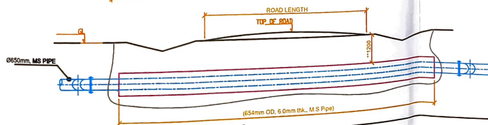
SECTION TYPICAL DETAIL OF ROAD CROSSING
